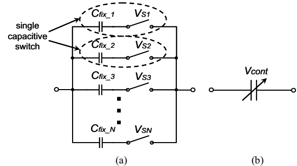
Fig. 1. (a) Schematic of the capacitive switch bank composed of N capacitive switches. (b) Schematic of the varactor.
